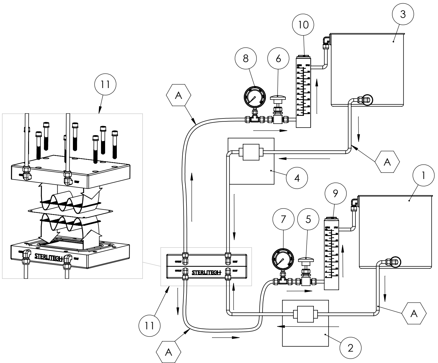
Direct Contact Membrane Distillation Flow Diagram
