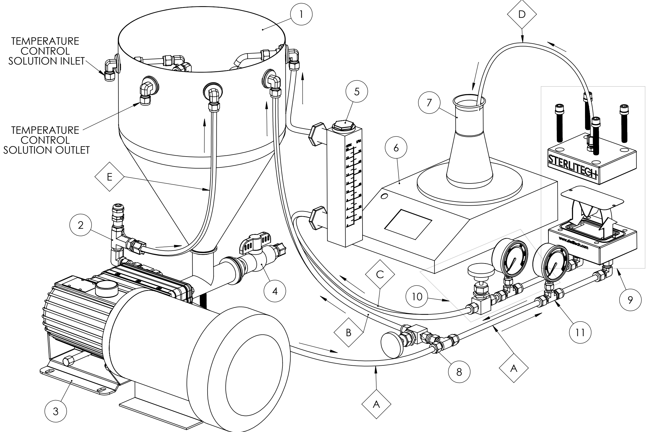
CF042A FLOW DIAGRAM
